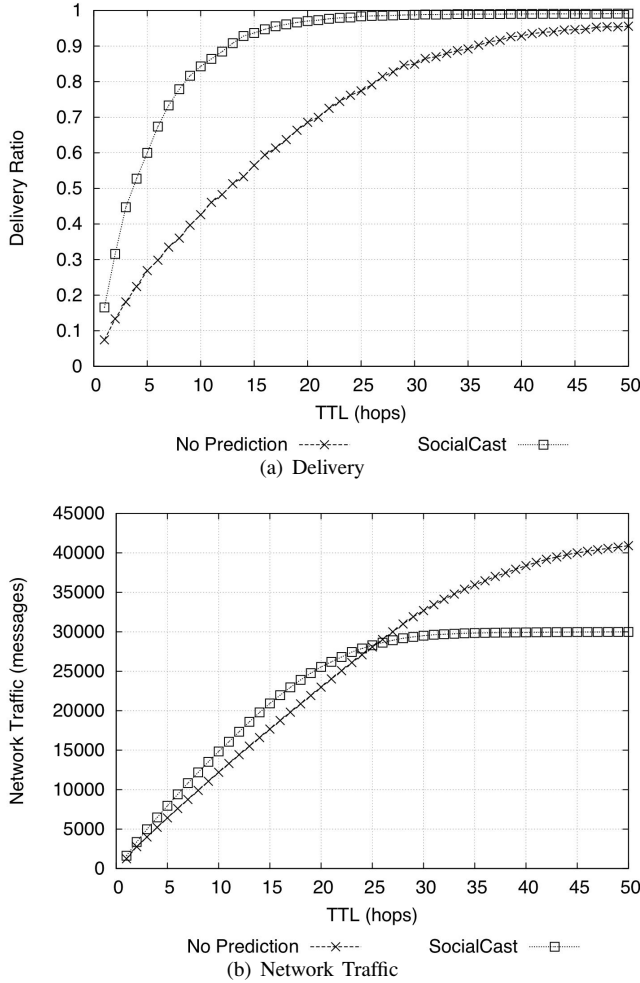
Fig. 5. Delivery and overhead against time-to-live.
