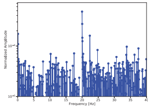
Fig. 3: FFT of the magnetometer traces while playing (on high volume) pure tones at 20Hz .
