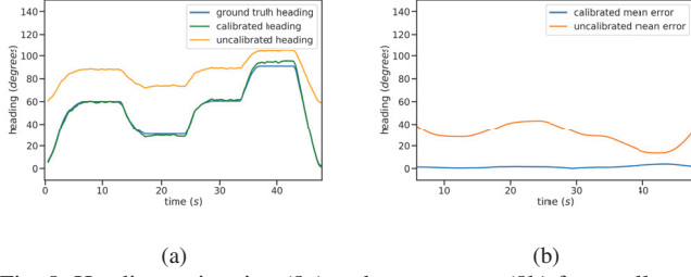
Fig. 8: Heading estimation (8a) and mean errors (8b) for small angles.
