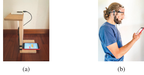
Fig. 7: Setup used to benchmark the proposed calibration technique (7a) and volunteer wearing the Arduino as if they were earbuds (7b). This is the setup used for our in-the-wild use test.
