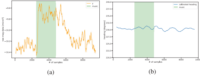
Fig. 2: Impact of audio streaming on calibrated magnetometers.
