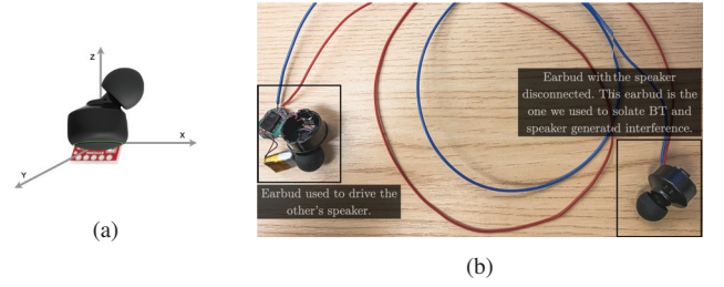
Fig. 1: Basic system setup (Figure 1a) and setup used to isolate the interference generated by BT streaming and speaker (Figure 1b).
