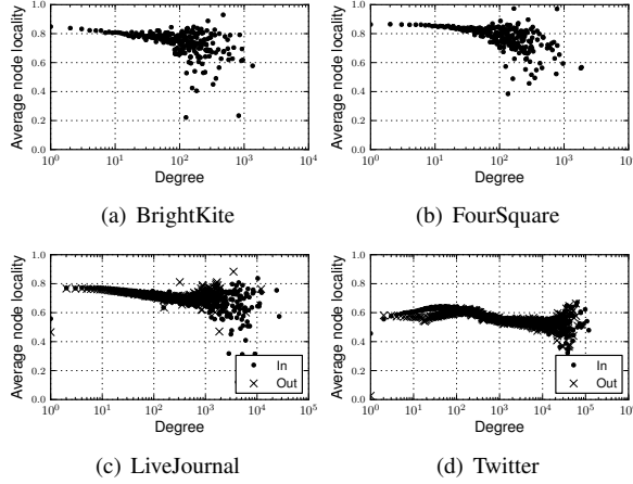
Figure 4: Average node locality as a function of node degree. For directed networks the relationship is shown both for incoming and outgoing links.
