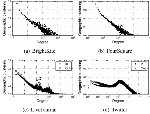
Figure 6: Average geographic clustering coefficient as a function of node degree. For directed networks the relationship is shown both for in- and out-degree.
